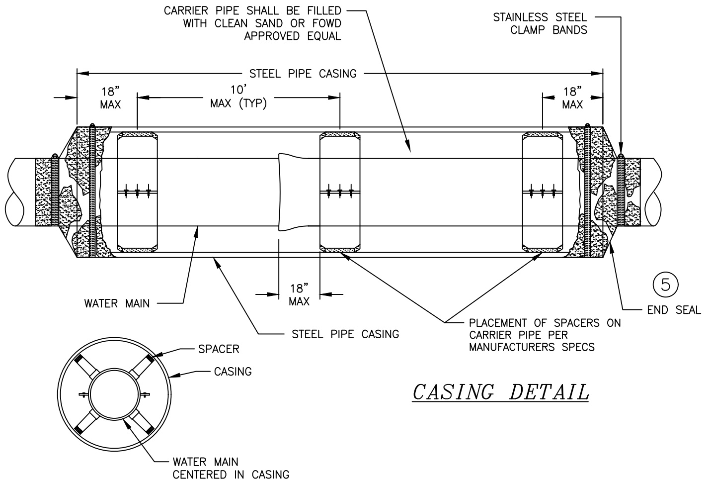
CROSS SECTION
